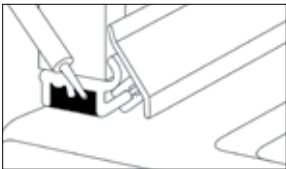
Seal one Sealant between seal & tray
