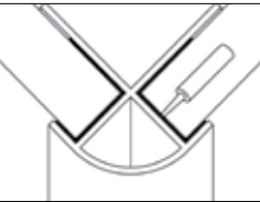
External corner Used on all external 90° corners
