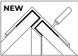
External corner Used on all external 90° corners
