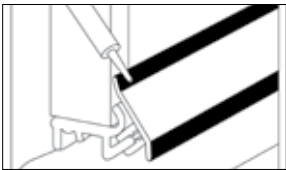
Seals three & four Top & bottom seal
