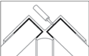
Internal corner Used on all internal 90° corners
