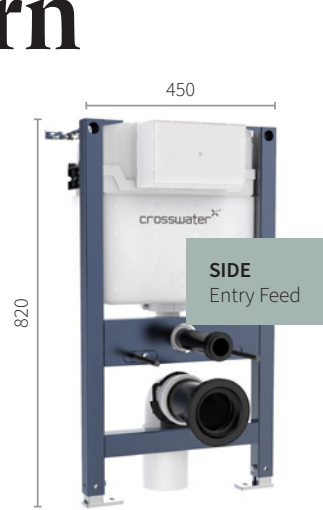
0.82m Toilet Frame Frame A Depth range: Top flush: 170-200mm Front flush: 190-260mm Under window or in furniture unit
